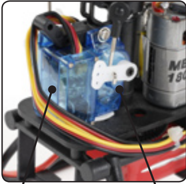
Elevator servo
