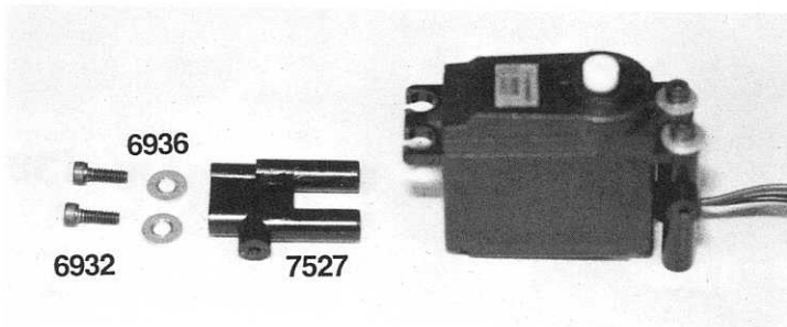
□ #6932 4-40 x 5/16 ○ #6936 #4 flat washer aluminum Fig. 133
